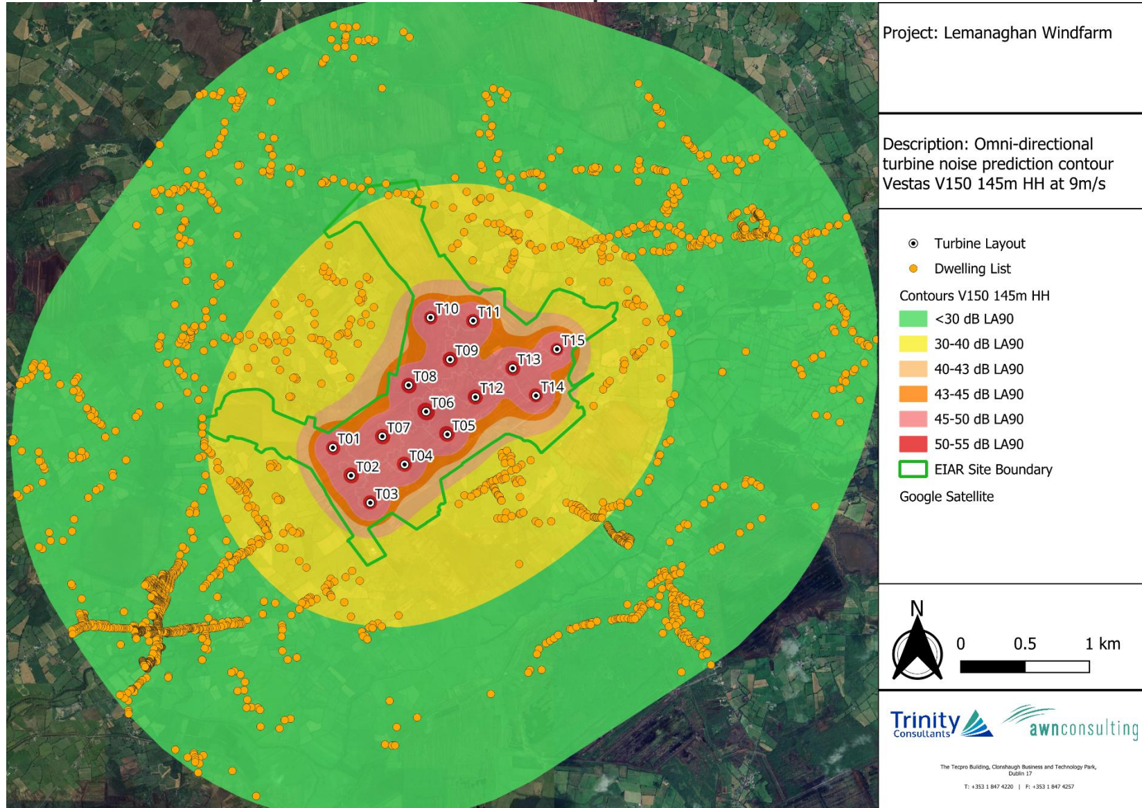
Figure A12-1 Omni Directional noise prediction contour V150 145m HH
